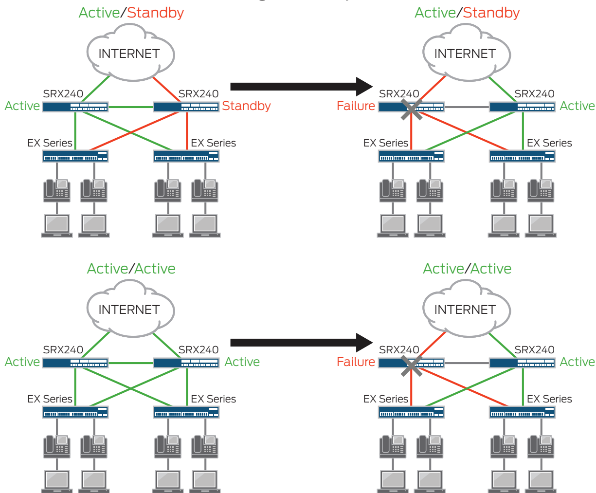
Figure 2: High availability
